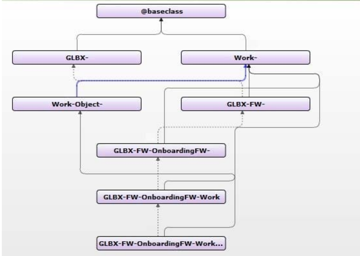
Class Inheritance Diagram for GLBX-FW-OnboardingFW-Work-EquipmentRequest
